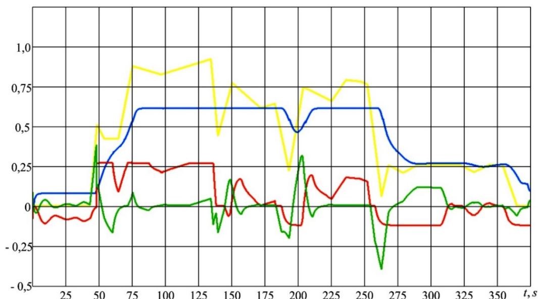
Fig. 2.12. Characteristics of capacities in different DEPC parts: — maximum load power corresponds to the value of 1000 kW; — maximum capacity in ESS corresponds to the value of 10 kW; — maximum capacity in ESS corresponds to the value of 20 kW; — maximum capacity in DC-Link corresponds to the value of 300 kW.
