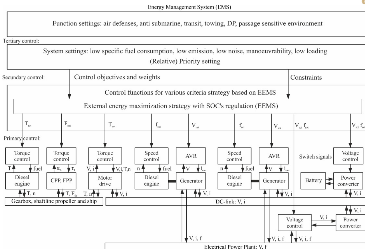
Fig. 3.17. Block diagram of the control strategy of the SPP CPC for the criterion of the maximum of alternative energy and the regulation of the battery charge level BSPS: X_{set} – setting; T – thrust (moment); F – force of propeller; f – voltage frequency; V – voltage; n – speed of rotation of MSDG; i_{exc} – current of excitation of MSDG; i – current; \tau_T – resultant projection of the vector of effort on the plane of the vessel; \alpha_A – angle of position of the THRs
