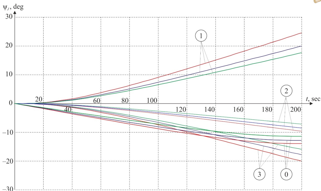
Fig. 1.5. Diagrams of dependency of yaw angle of the ship, type Supply Vessel, length 76 m, in the time function: 0÷3 – numbers of appropriate configurations (1.17), (1.18), (1.19), (1.20): — — — — — mutual perpendicular axis location of the main and auxiliary pods with unchanged values of step ratios and thrusts coefficients; — — — — — mutual perpendicular axis location of the main and auxiliary pods with regulated values of step ratios and thrusts coefficients; — — — — — the optimal location of the axes of the main and auxiliary pods with values of step ratios and thrusts coefficients that meet the criterion of minimum change in the XY -coordinates of the ship.
