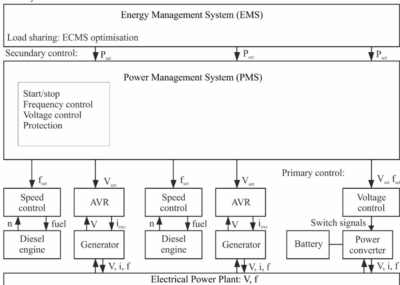
Control strategy for hybrid power supply with ECMS
